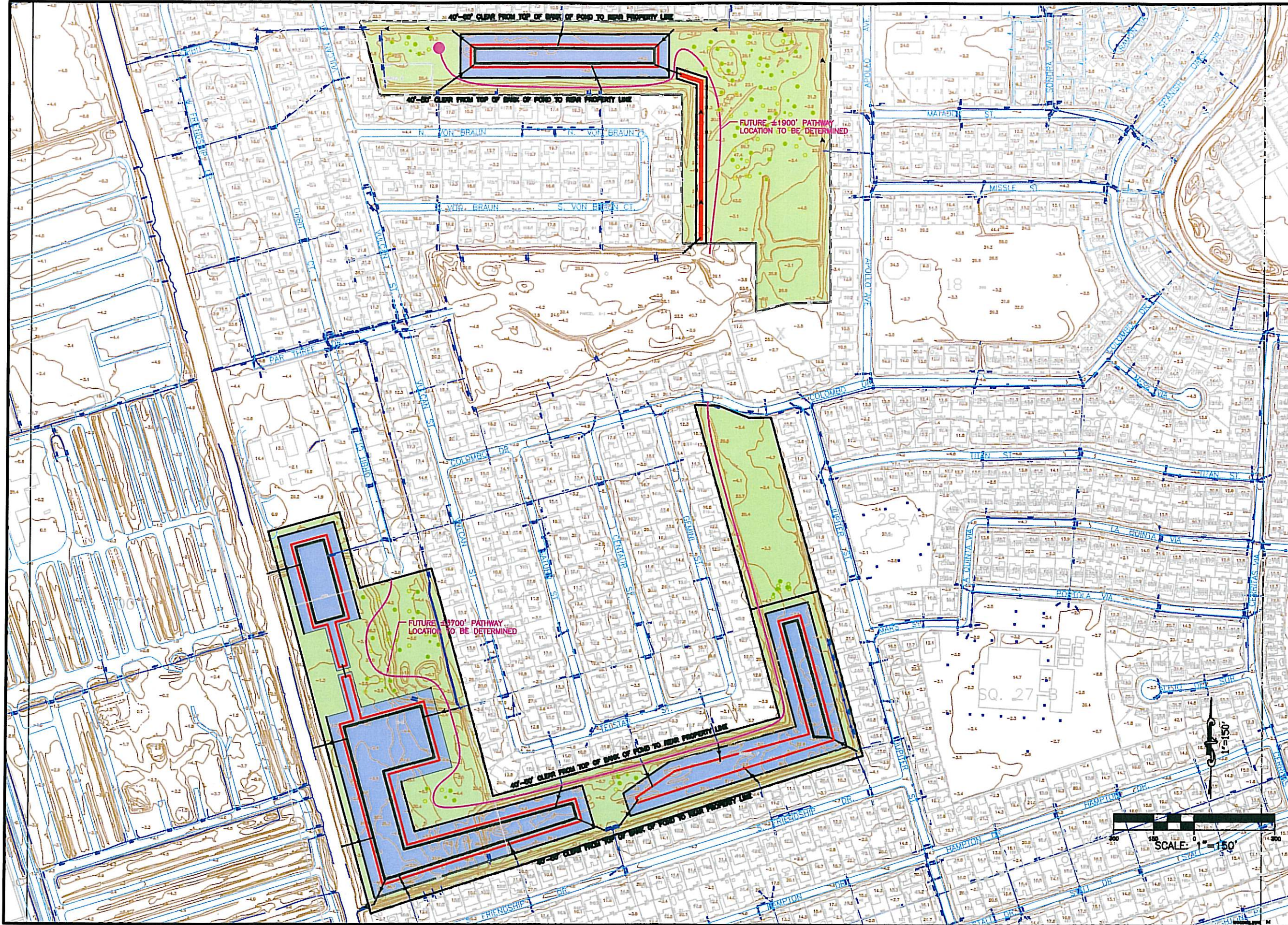
SITE PLAN (WEST DETENTION POND ALTERNATIVE)
